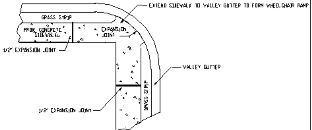
WHEELCHAIR RAMP IN VALLEY GUTTER
