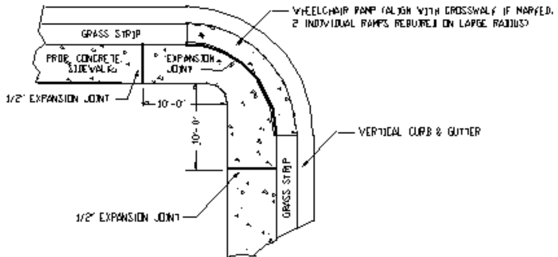
WHEELCHAIR RAMP IN VERTICAL CURB & GUTTER
