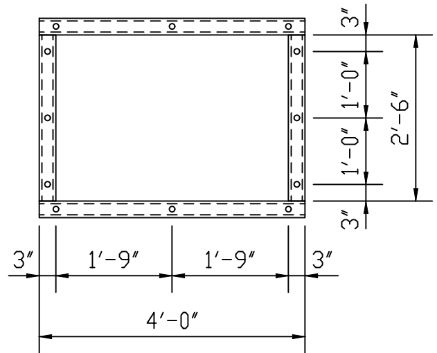
PLAN OF 3" C FRAME
