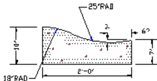
2'-0" VALLEY GUTTER
