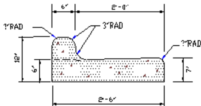
2'-6" CURB AND GUTTER
