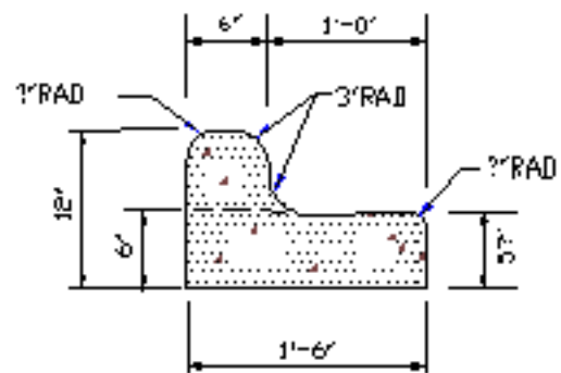
1'-6" CURB AND GUTTER
