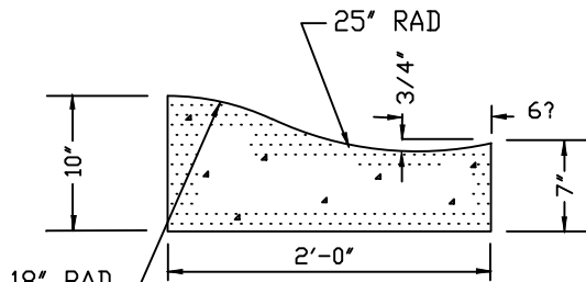
2'-0" VALLEY GUTTER
