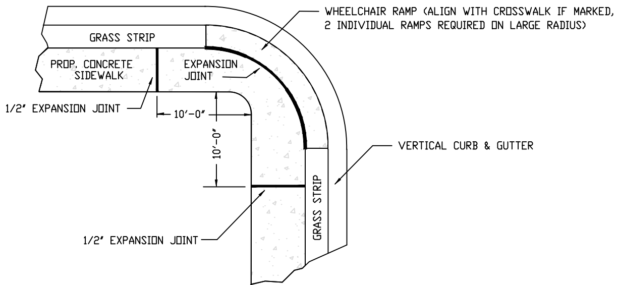
WHEELCHAIR RAMP IN VERTICAL CURB & GUTTER
