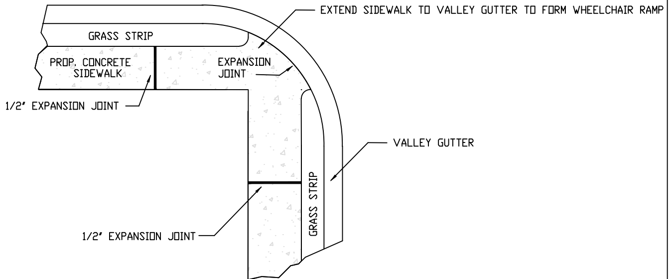
WHEELCHAIR RAMP IN VALLEY GUTTER
